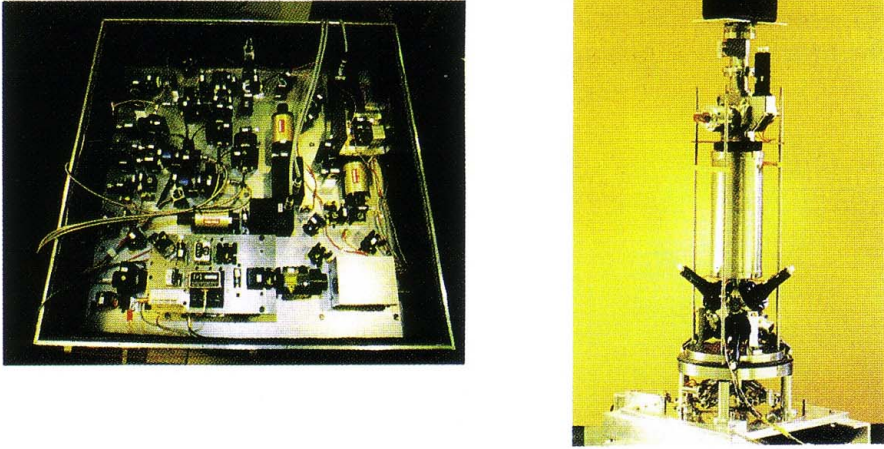
Figure 11. The microgravity clock prototype. The left part is the 60 cm \times 60 cm \times 15 cm optical bench containing the diode laser sources and the various optical components. The right part is the clock itself (about one meter long) containing the optical molasses, the microwave cavity and the detection region.
