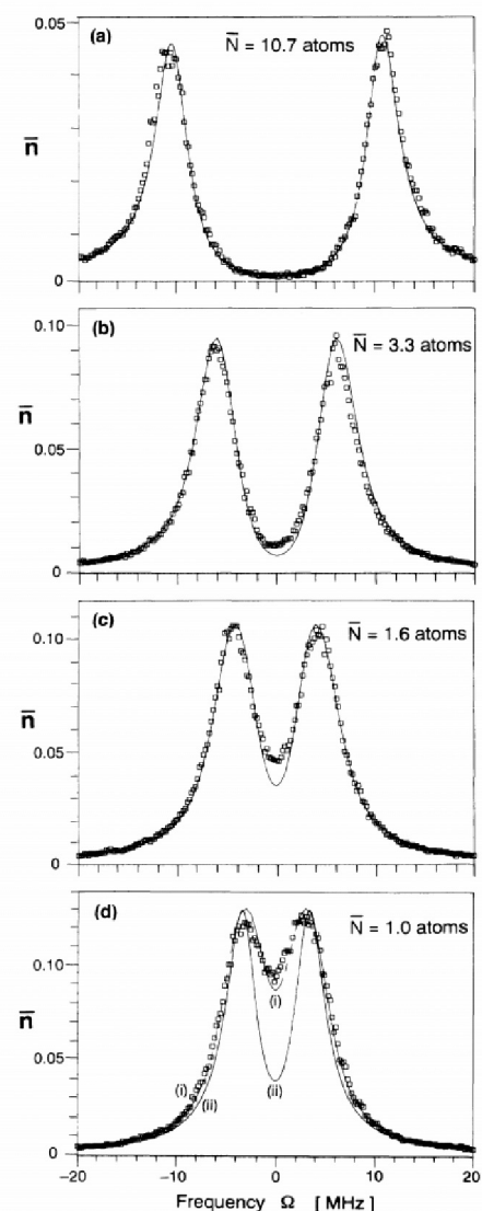
FIG. 2. Intracavity photon number \bar{n} vs probe frequency \Omega for four values of \bar{N} and with \omega_c \simeq \omega_A . Curves in (a)–(c) and curve i in (d) are theoretical fits to the data including fluctuations in atomic number and position. Curve ii in (d) is from Eq. (1) for a single intracavity atom with optimum coupling g_0 .
